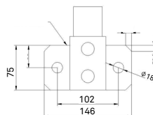
F2 - Face Mount (2 Fixings)
