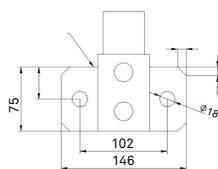
F2 - Face Mount (2 Fixings)
