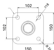
T4 - Top Mount (4 Fixings)
